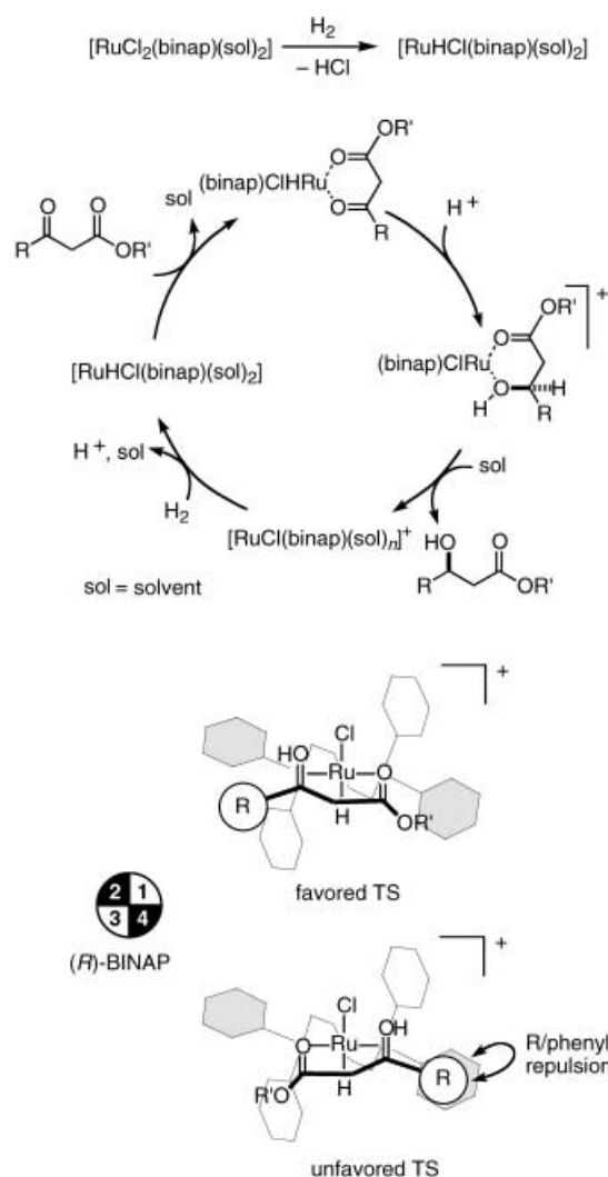
Figure 8. Mechanism of (R)-BINAP–Ru catalyzed hydrogenation of \beta -keto esters.
