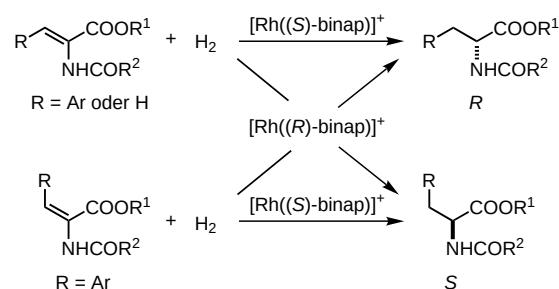
Scheme 4. Asymmetric hydrogenation of \alpha -(acylamino)acrylic acids catalyzed by BINAP–Rh complexes.
