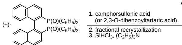
Scheme 2. Access to enantiomerically pure BINAP.
