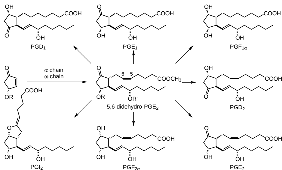
Scheme 14. Three-component synthesis of prostaglandins. \alpha chain = \text{ICH}_2\text{C}\equiv\text{C}(\text{CH}_2)_3\text{COOCH}_3 ; \omega chain = (E,S)\text{-LiCH=CHCH(OR')(\text{CH}_2)_4\text{CH}_3 .
