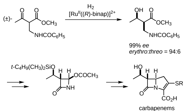
Scheme 10. Stereoselective synthesis of carbapenem antibiotics.
