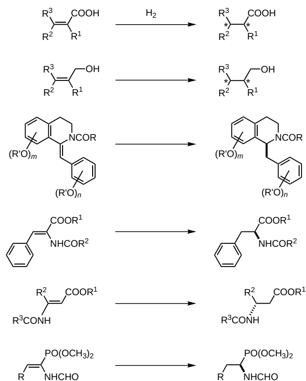
Scheme 5. Asymmetric hydrogenation of functionalized olefins catalyzed by ( S )-BINAP–Ru dicarboxylates.
