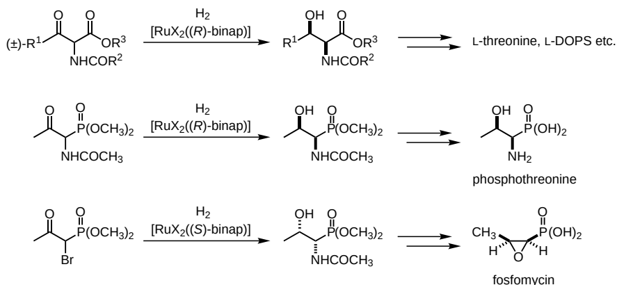
Scheme 9. Asymmetric hydrogenation by dynamic kinetic resolution. X = Cl, Br.
