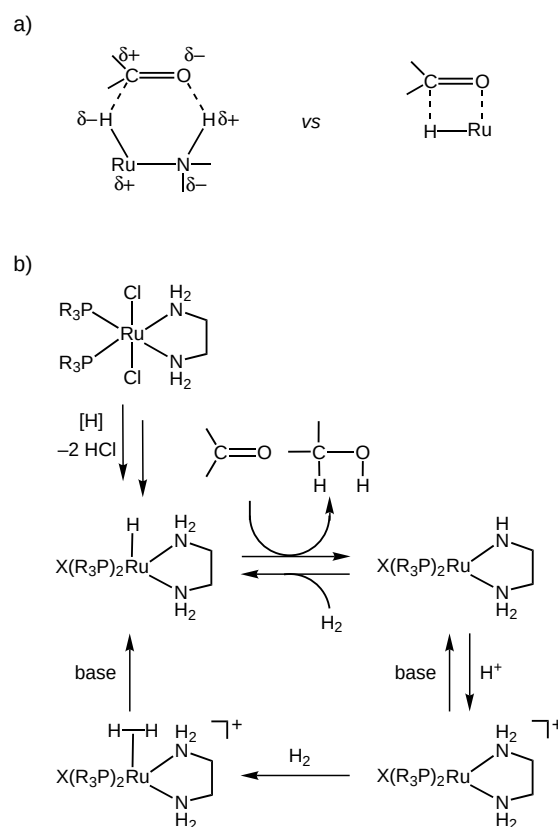
Figure 9. a) Nonclassical metal–ligand bifunctional mechanism and conventional [2+2] mechanism. b) Catalytic cycle of hydrogenation of ketones with a [RuCl 2 (PR 3 ) 2 (NH 2 CH 2 CH 2 NH 2 )]/strong base combined system in 2-propanol. X = H, OR, etc.
