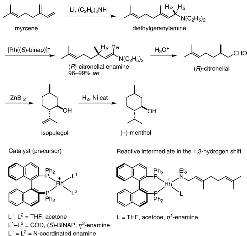
Scheme 3. Takasago menthol synthesis. COD = 1,5-cyclooctadiene.
